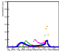
800 GeV incident in L2
