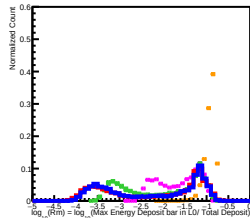
800 GeV incident in L3
