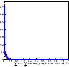
100 GeV incident in L5
