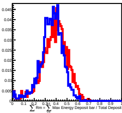
100 GeV incident in L11
