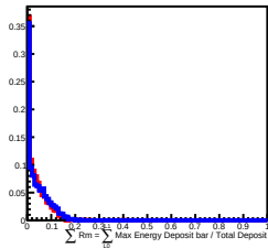
100 GeV incident in L6
