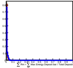
200 GeV incident in L5
