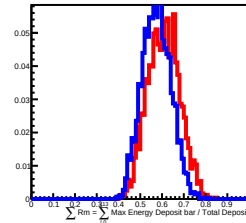
200 GeV incident in L13
