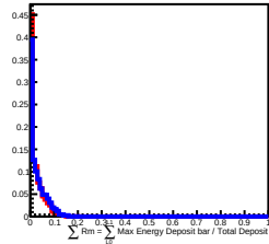
200 GeV incident in L6
