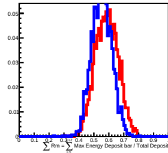
200 GeV incident in L12
