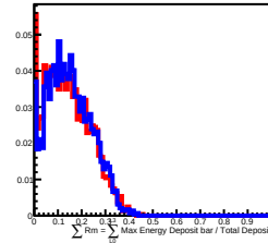
200 GeV incident in L8
