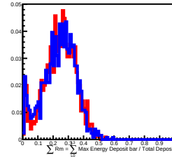
20 GeV incident in L8
