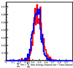
20 GeV incident in L10
