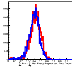
20 GeV incident in L12
