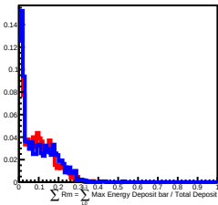
20 GeV incident in L6
