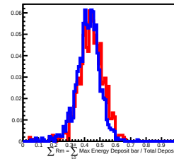
20 GeV incident in L13
