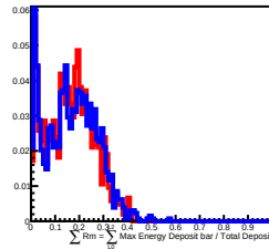
20 GeV incident in L7
