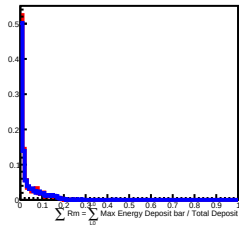
20 GeV incident in L5
