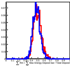
20 GeV incident in L11
