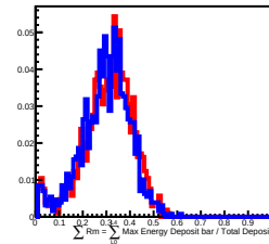
20 GeV incident in L9
