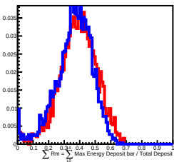
300 GeV incident in L11
