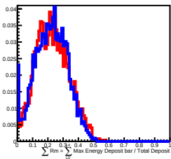
300 GeV incident in L9
