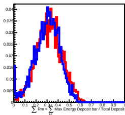
300 GeV incident in L10
