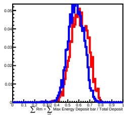
300 GeV incident in L12
