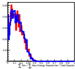
300 GeV incident in L8
