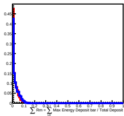
300 GeV incident in L6
