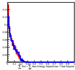
300 GeV incident in L7
