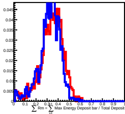
30 GeV incident in L10
