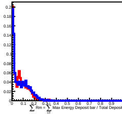
30 GeV incident in L6
