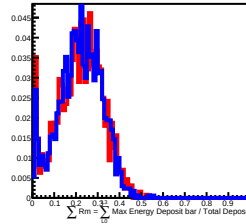
30 GeV incident in L8
