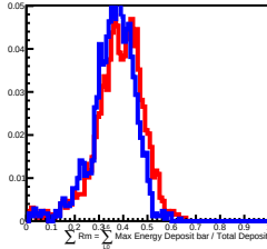
30 GeV incident in L11
