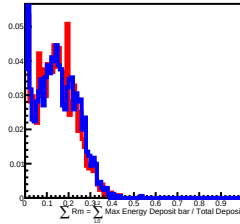
30 GeV incident in L7
