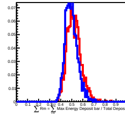
30 GeV incident in L13
