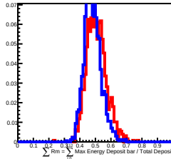
30 GeV incident in L12
