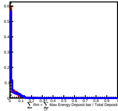
30 GeV incident in L5
