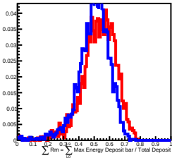
400 GeV incident in L9
