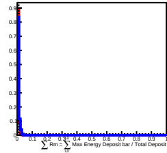
400 GeV incident in L5
