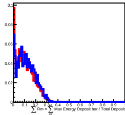
60 GeV incident in L7
