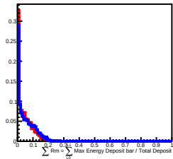
60 GeV incident in L6
