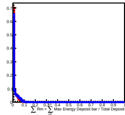
60 GeV incident in L5
