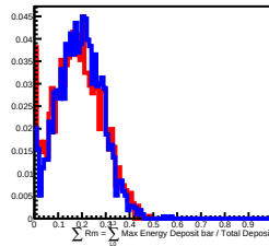
60 GeV incident in L8
