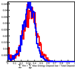
60 GeV incident in L10
