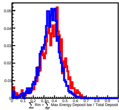
60 GeV incident in L11
