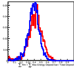
60 GeV incident in L12
