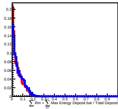
700 GeV incident in L7
