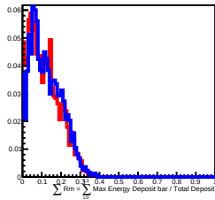
700 GeV incident in L8
