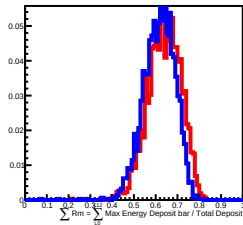
700 GeV incident in L12
