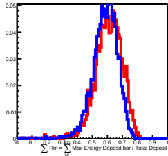
700 GeV incident in L11
