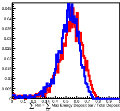
700 GeV incident in L9
