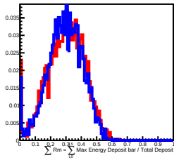
700 GeV incident in L10
