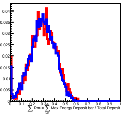
800 GeV incident in L10
