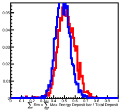
80 GeV incident in L11
