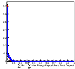
80 GeV incident in L5
