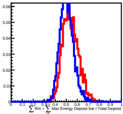
80 GeV incident in L12
