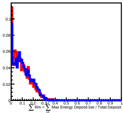
80 GeV incident in L7
