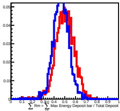
80 GeV incident in L10
