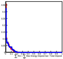
80 GeV incident in L6
