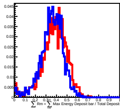
90 GeV incident in L11
