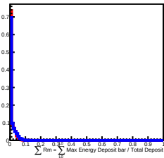
90 GeV incident in L5
