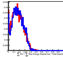
90 GeV incident in L8
