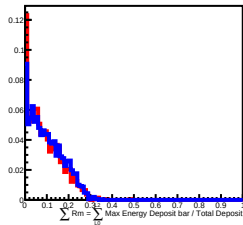
90 GeV incident in L7
