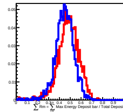
90 GeV incident in L9
