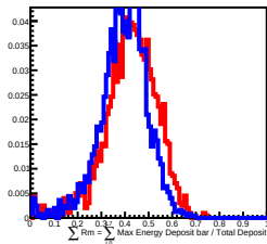
90 GeV incident in L12
