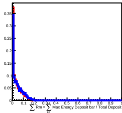
90 GeV incident in L6
