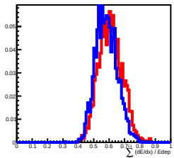
Deposit Energy[63.10GeV, 100.00GeV] in L11
