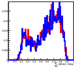
Deposit Energy[630.96GeV, 1000.00GeV] in L6
