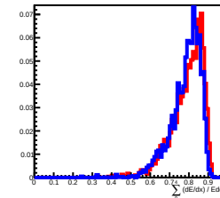
Deposit Energy[630.96GeV, 1000.00GeV] in L9
