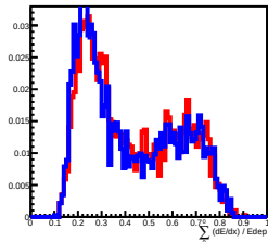
Deposit Energy[630.96GeV, 1000.00GeV] in L5
