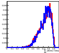
Deposit Energy[630.96GeV, 1000.00GeV] in L7
