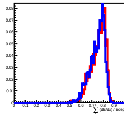
Deposit Energy[1584.89GeV, 2511.89GeV] in L9
