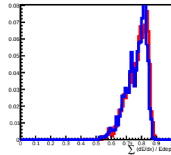
Deposit Energy[2511.89GeV, 3981.07GeV] in L13
