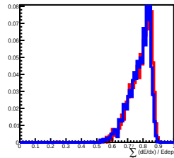
Deposit Energy[2511.89GeV, 3981.07GeV] in L12
