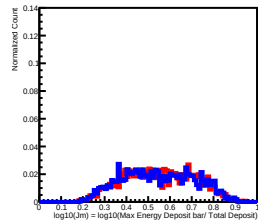
Deposit Energy[25.12GeV, 39.81GeV] in L0
