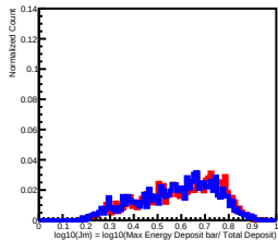
Deposit Energy[25.12GeV, 39.81GeV] in L1
