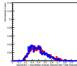
Deposit Energy[25.12GeV, 39.81GeV] in L8
