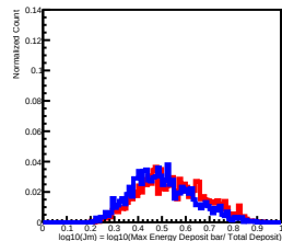
Deposit Energy[25.12GeV, 39.81GeV] in L5
