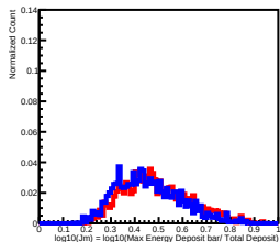
Deposit Energy[25.12GeV, 39.81GeV] in L6
