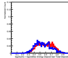
Deposit Energy[25.12GeV, 39.81GeV] in L4
