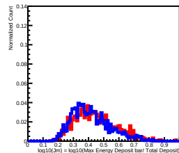
Deposit Energy[25.12GeV, 39.81GeV] in L7
