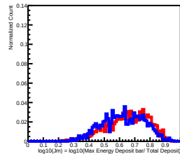
Deposit Energy[25.12GeV, 39.81GeV] in L2
