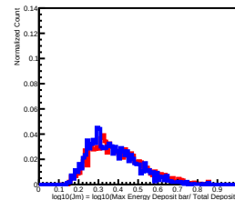
Deposit Energy[25.12GeV, 39.81GeV] in L9
