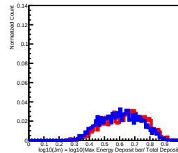
Deposit Energy[25.12GeV, 39.81GeV] in L3
