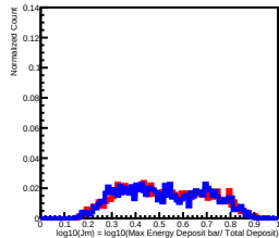
Deposit Energy[63.10GeV, 100.00GeV] in L5
