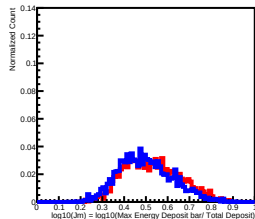
Deposit Energy[63.10GeV, 100.00GeV] in L7
