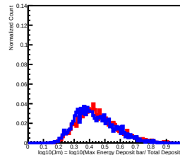
Deposit Energy[63.10GeV, 100.00GeV] in L9
