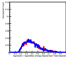
Deposit Energy[63.10GeV, 100.00GeV] in L12
