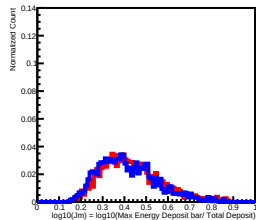
Deposit Energy[63.10GeV, 100.00GeV] in L10
