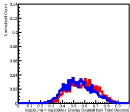
Deposit Energy[63.10GeV, 100.00GeV] in L6
