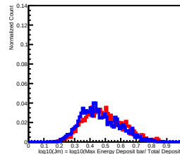
Deposit Energy[63.10GeV, 100.00GeV] in L8
