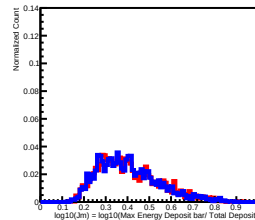
Deposit Energy[63.10GeV, 100.00GeV] in L13
