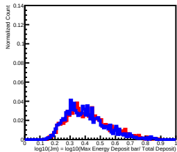
Deposit Energy[63.10GeV, 100.00GeV] in L11
