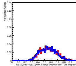
Deposit Energy[630.96GeV, 1000.00GeV] in L13
