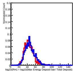
Deposit Energy[100.00GeV, 158.49GeV] in L10
