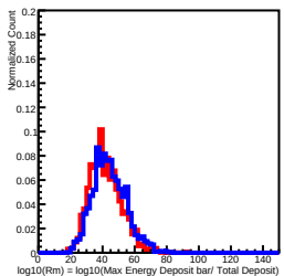
Deposit Energy[100.00GeV, 158.49GeV] in L9
