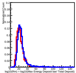
Deposit Energy[100.00GeV, 158.49GeV] in L2
