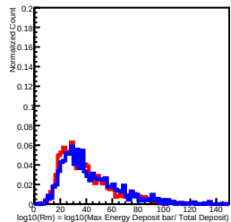
Deposit Energy[100.00GeV, 158.49GeV] in L0
