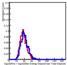
Deposit Energy[100.00GeV, 158.49GeV] in L13
