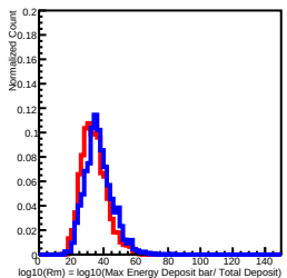
Deposit Energy[100.00GeV, 158.49GeV] in L12
