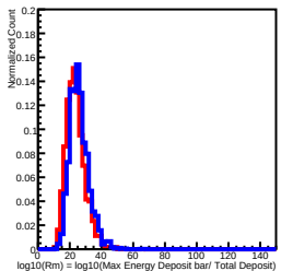
Deposit Energy[100.00GeV, 158.49GeV] in L4
