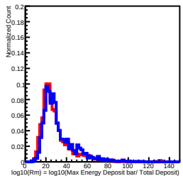
Deposit Energy[100.00GeV, 158.49GeV] in L1
