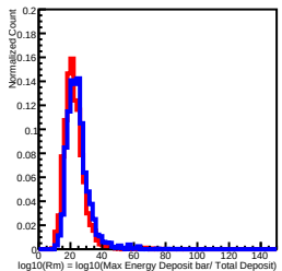
Deposit Energy[100.00GeV, 158.49GeV] in L3
