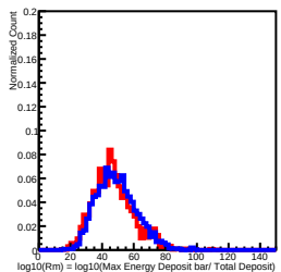
Deposit Energy[100.00GeV, 158.49GeV] in L11
