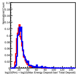
Deposit Energy[158.49GeV, 251.19GeV] in L2
