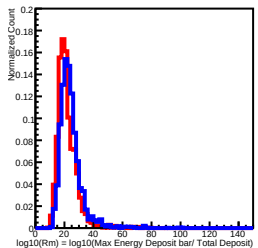
Deposit Energy[158.49GeV, 251.19GeV] in L3
