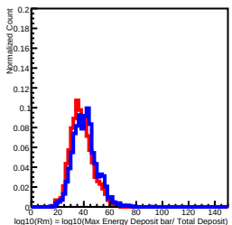
Deposit Energy[158.49GeV, 251.19GeV] in L9
