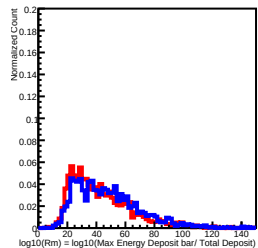
Deposit Energy[158.49GeV, 251.19GeV] in L0
