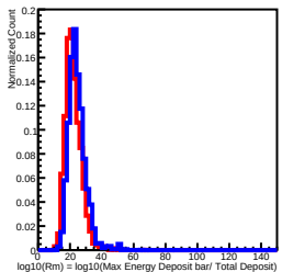
Deposit Energy[158.49GeV, 251.19GeV] in L4
