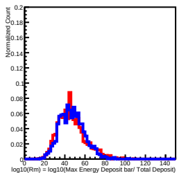
Deposit Energy[158.49GeV, 251.19GeV] in L13
