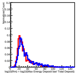
Deposit Energy[158.49GeV, 251.19GeV] in L1
