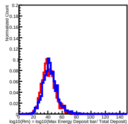
Deposit Energy[158.49GeV, 251.19GeV] in L10
