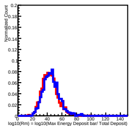
Deposit Energy[158.49GeV, 251.19GeV] in L11
