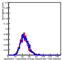
Deposit Energy[158.49GeV, 251.19GeV] in L12
