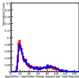
Deposit Energy[1584.89GeV, 2511.89GeV] in L2
