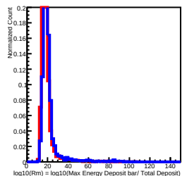
Deposit Energy[1584.89GeV, 2511.89GeV] in L5
