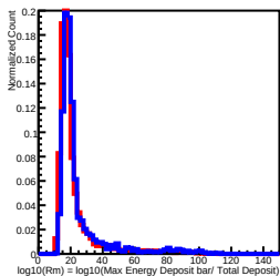
Deposit Energy[1584.89GeV, 2511.89GeV] in L4
