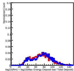
Deposit Energy[1584.89GeV, 2511.89GeV] in L0
