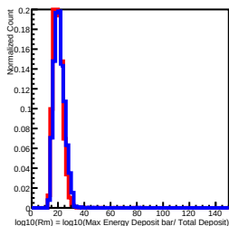
Deposit Energy[1584.89GeV, 2511.89GeV] in L7
