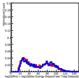
Deposit Energy[1584.89GeV, 2511.89GeV] in L1
