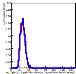
Deposit Energy[1584.89GeV, 2511.89GeV] in L10
