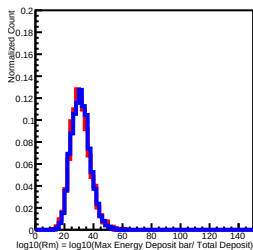
Deposit Energy[1584.89GeV, 2511.89GeV] in L13
