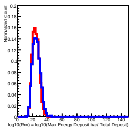
Deposit Energy[1584.89GeV, 2511.89GeV] in L9
