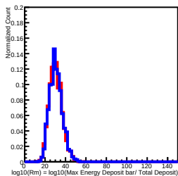
Deposit Energy[1584.89GeV, 2511.89GeV] in L12
