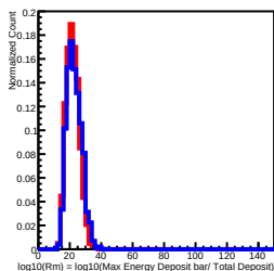
Deposit Energy[1584.89GeV, 2511.89GeV] in L8
