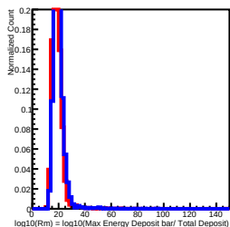
Deposit Energy[1584.89GeV, 2511.89GeV] in L6
