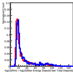
Deposit Energy[1584.89GeV, 2511.89GeV] in L3
