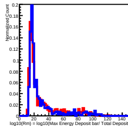
Deposit Energy[3981.07GeV, 6309.57GeV] in L3
