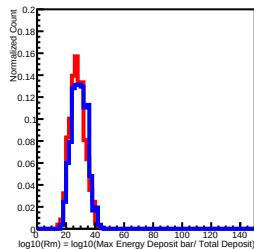
Deposit Energy[3981.07GeV, 6309.57GeV] in L12
