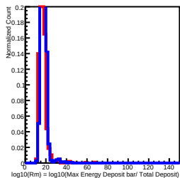
Deposit Energy[3981.07GeV, 6309.57GeV] in L6
