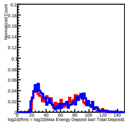
Deposit Energy[3981.07GeV, 6309.57GeV] in L1
