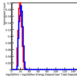
Deposit Energy[3981.07GeV, 6309.57GeV] in L8
