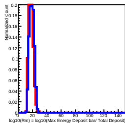
Deposit Energy[3981.07GeV, 6309.57GeV] in L7
