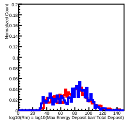
Deposit Energy[3981.07GeV, 6309.57GeV] in L0
