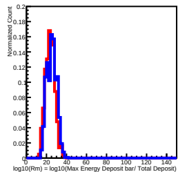
Deposit Energy[3981.07GeV, 6309.57GeV] in L10
