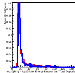
Deposit Energy[3981.07GeV, 6309.57GeV] in L4
