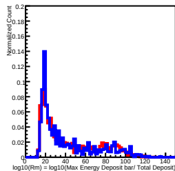
Deposit Energy[3981.07GeV, 6309.57GeV] in L2
