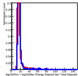
Deposit Energy[3981.07GeV, 6309.57GeV] in L5
