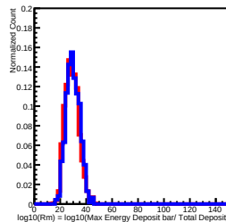
Deposit Energy[3981.07GeV, 6309.57GeV] in L13
