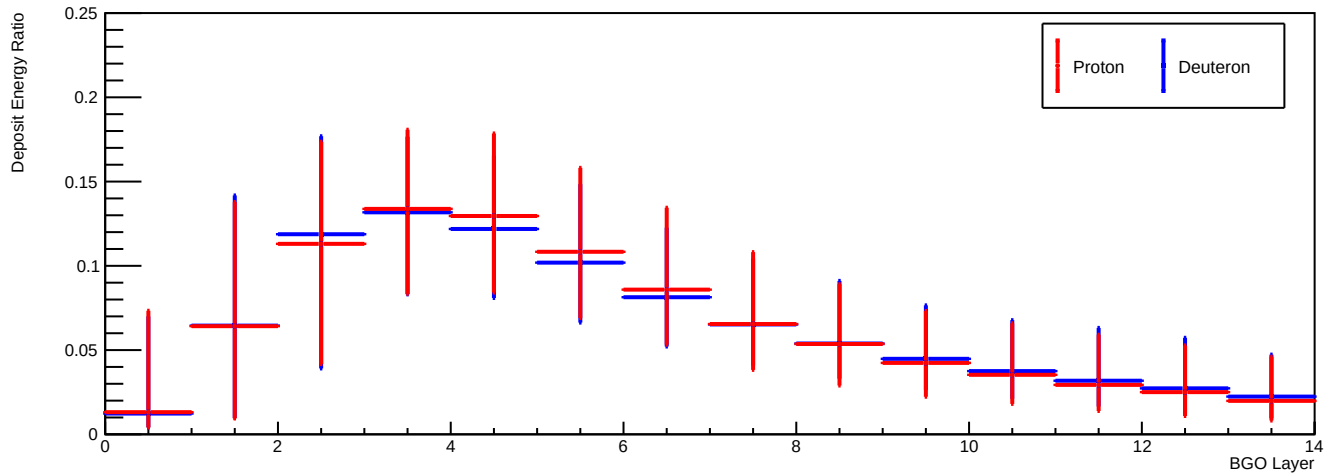
Deposit Energy [15.85GeV, 25.12GeV] GeV
