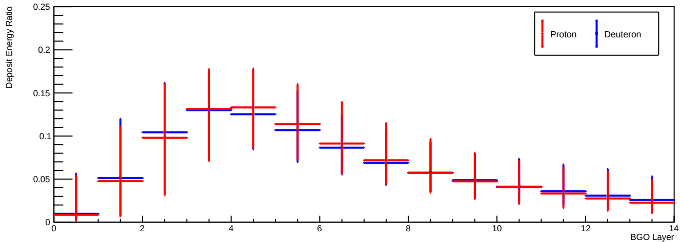
Deposit Energy [25.12GeV, 39.81GeV] GeV
