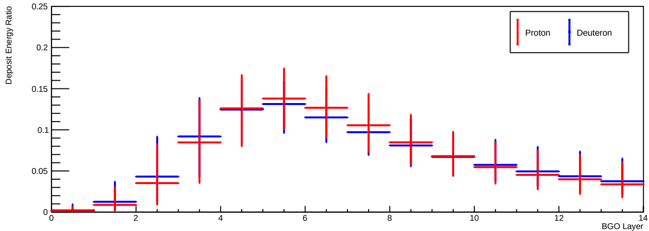
Deposit Energy [398.11GeV, 630.96GeV] GeV
