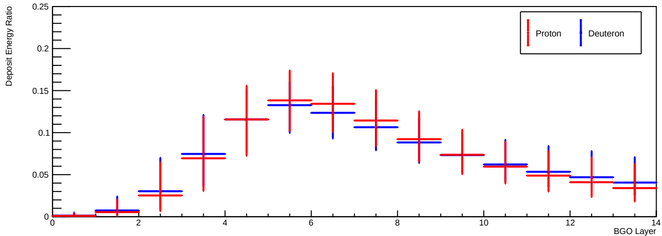
Deposit Energy [1000.00GeV, 1584.89GeV] GeV
