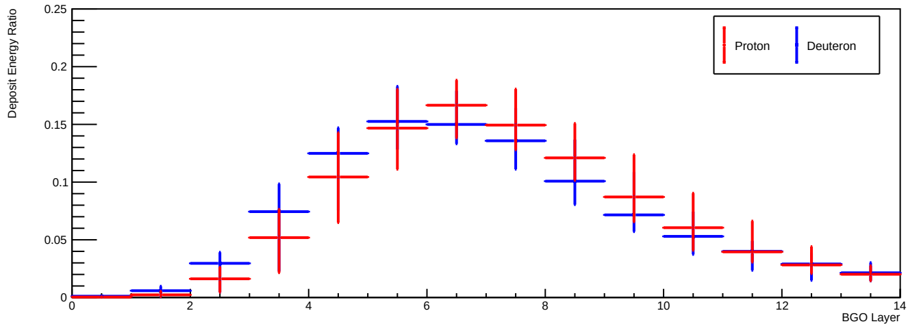
Deposit Energy [6309.57GeV, 10000.00GeV] GeV
