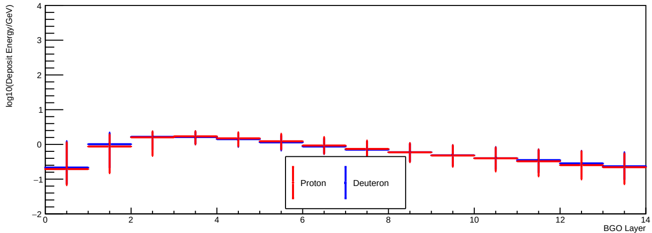
Deposit Energy [10.00GeV, 15.85GeV] GeV
