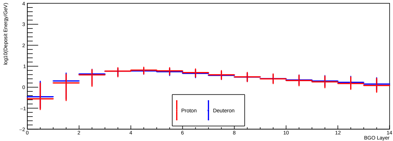
Deposit Energy [39.81GeV, 63.10GeV] GeV
