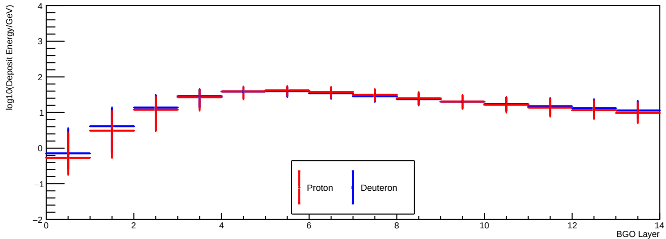
Deposit Energy [251.19GeV, 398.11GeV] GeV
