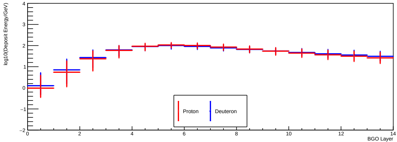
Deposit Energy [630.96GeV, 1000.00GeV] GeV
