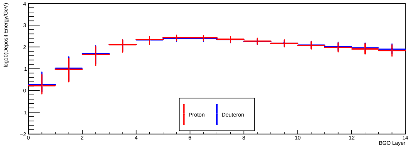
Deposit Energy [1584.89GeV, 2511.89GeV] GeV
