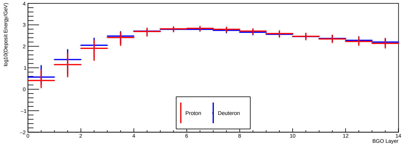
Deposit Energy [3981.07GeV, 6309.57GeV] GeV
