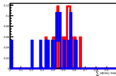
Deposit Energy[100.00GeV, 158.49GeV] in L13
