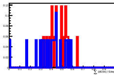
Deposit Energy[100.00GeV, 158.49GeV] in L12
