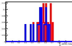
Deposit Energy[100.00GeV, 158.49GeV] in L11
