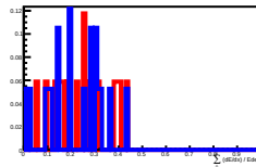
Deposit Energy[100.00GeV, 158.49GeV] in L9
