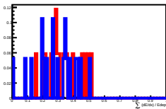
Deposit Energy[100.00GeV, 158.49GeV] in L10
