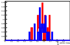
Deposit Energy[251.19GeV, 398.11GeV] in L10
