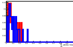
Deposit Energy[251.19GeV, 398.11GeV] in L8
