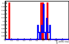
Deposit Energy[398.11GeV, 630.96GeV] in L11
