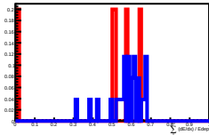
Deposit Energy[398.11GeV, 630.96GeV] in L10
