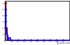
Deposit Energy[398.11GeV, 630.96GeV] in L6
