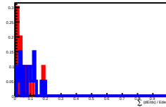
Deposit Energy[1584.89GeV, 2511.89GeV] in L8
