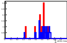
Deposit Energy[1584.89GeV, 2511.89GeV] in L10
