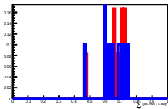
Deposit Energy[2511.89GeV, 3981.07GeV] in L11
