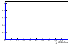
Deposit Energy[2511.89GeV, 3981.07GeV] in L5
