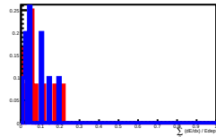
Deposit Energy[2511.89GeV, 3981.07GeV] in L8
