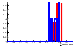
Deposit Energy[2511.89GeV, 3981.07GeV] in L13
