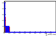
Deposit Energy[2511.89GeV, 3981.07GeV] in L7
