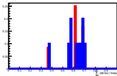
Deposit Energy[2511.89GeV, 3981.07GeV] in L10
