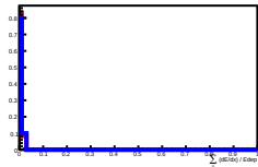
Deposit Energy[2511.89GeV, 3981.07GeV] in L6
