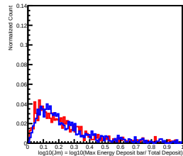
Deposit Energy[10.00GeV, 15.85GeV] in L10
