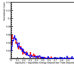
Deposit Energy[10.00GeV, 15.85GeV] in L13
