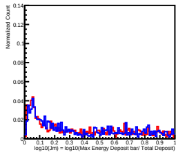
Deposit Energy[10.00GeV, 15.85GeV] in L6
