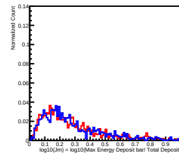
Deposit Energy[10.00GeV, 15.85GeV] in L9
