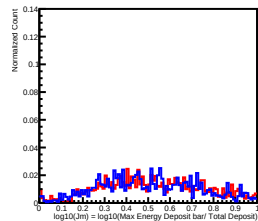
Deposit Energy[10.00GeV, 15.85GeV] in L5
