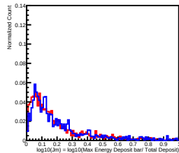
Deposit Energy[10.00GeV, 15.85GeV] in L12
