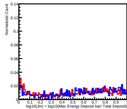
Deposit Energy[10.00GeV, 15.85GeV] in L7
