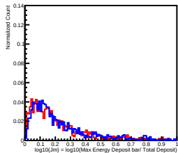
Deposit Energy[10.00GeV, 15.85GeV] in L11
