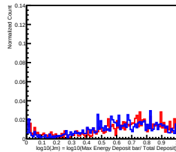
Deposit Energy[10.00GeV, 15.85GeV] in L8
