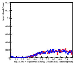
Deposit Energy[100.00GeV, 158.49GeV] in L6
