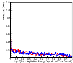
Deposit Energy[100.00GeV, 158.49GeV] in L7
