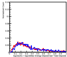
Deposit Energy[100.00GeV, 158.49GeV] in L12
