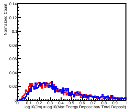
Deposit Energy[100.00GeV, 158.49GeV] in L11
