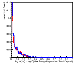
Deposit Energy[100.00GeV, 158.49GeV] in L5
