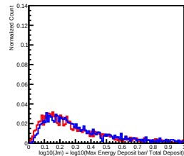
Deposit Energy[100.00GeV, 158.49GeV] in L13
