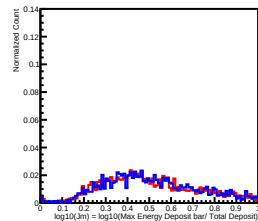
Deposit Energy[100.00GeV, 158.49GeV] in L8
