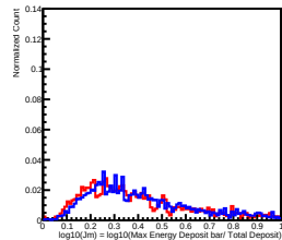
Deposit Energy[100.00GeV, 158.49GeV] in L10
