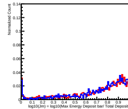
Deposit Energy[100.00GeV, 158.49GeV] in L9
