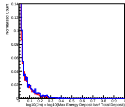
Deposit Energy[158.49GeV, 251.19GeV] in L0
