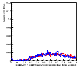
Deposit Energy[158.49GeV, 251.19GeV] in L7
