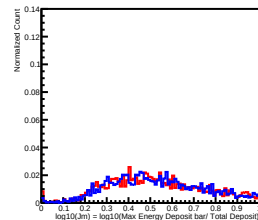
Deposit Energy[158.49GeV, 251.19GeV] in L8
