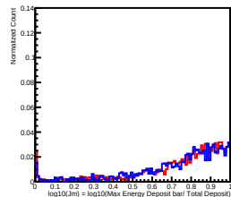
Deposit Energy[158.49GeV, 251.19GeV] in L5
