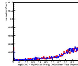
Deposit Energy[158.49GeV, 251.19GeV] in L4
