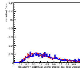
Deposit Energy[158.49GeV, 251.19GeV] in L9
