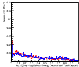
Deposit Energy[158.49GeV, 251.19GeV] in L2
