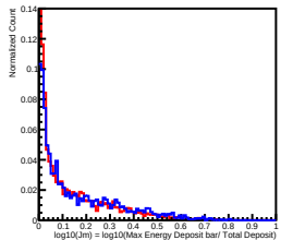
Deposit Energy[158.49GeV, 251.19GeV] in L1
