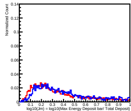
Deposit Energy[251.19GeV, 398.11GeV] in L12
