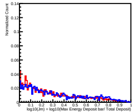
Deposit Energy[251.19GeV, 398.11GeV] in L7
