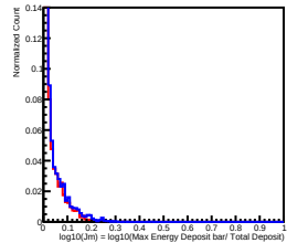
Deposit Energy[251.19GeV, 398.11GeV] in L5
