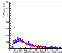
Deposit Energy[251.19GeV, 398.11GeV] in L13
