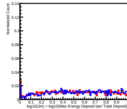
Deposit Energy[251.19GeV, 398.11GeV] in L8
