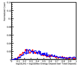
Deposit Energy[251.19GeV, 398.11GeV] in L10
