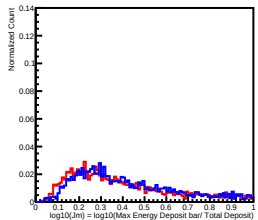
Deposit Energy[251.19GeV, 398.11GeV] in L11
