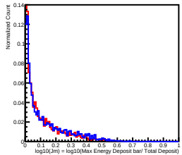
Deposit Energy[251.19GeV, 398.11GeV] in L6
