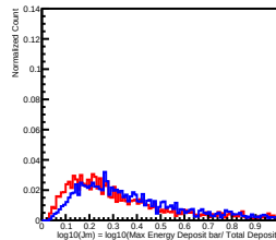
Deposit Energy[630.96GeV, 1000.00GeV] in L13
