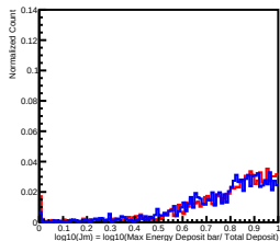
Deposit Energy[630.96GeV, 1000.00GeV] in L6
