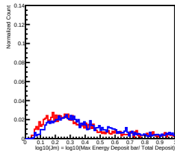
Deposit Energy[630.96GeV, 1000.00GeV] in L12
