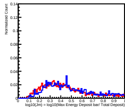
Deposit Energy[630.96GeV, 1000.00GeV] in L10
