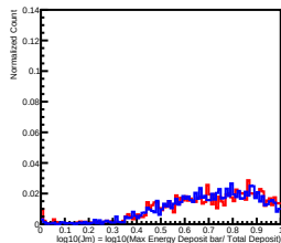
Deposit Energy[630.96GeV, 1000.00GeV] in L7
