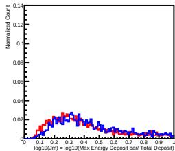
Deposit Energy[630.96GeV, 1000.00GeV] in L11
