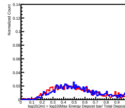
Deposit Energy[630.96GeV, 1000.00GeV] in L9
