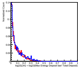
Deposit Energy[630.96GeV, 1000.00GeV] in L1
