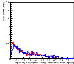
Deposit Energy[630.96GeV, 1000.00GeV] in L2
