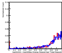
Deposit Energy[630.96GeV, 1000.00GeV] in L5
