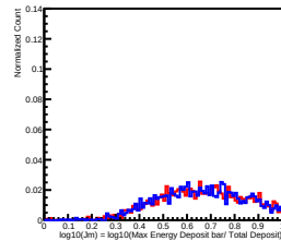
Deposit Energy[1584.89GeV, 2511.89GeV] in L8
