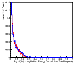
Deposit Energy[1584.89GeV, 2511.89GeV] in L1
