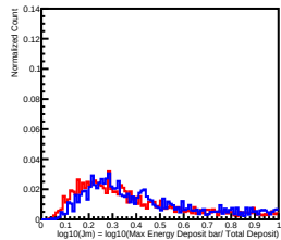
Deposit Energy[1584.89GeV, 2511.89GeV] in L12
