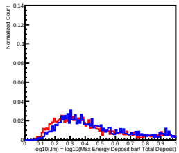
Deposit Energy[1584.89GeV, 2511.89GeV] in L11
