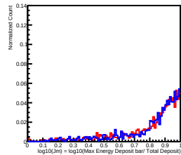
Deposit Energy[1584.89GeV, 2511.89GeV] in L5
