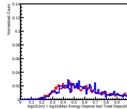
Deposit Energy[1584.89GeV, 2511.89GeV] in L9
