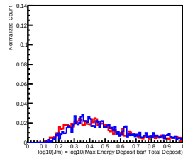
Deposit Energy[1584.89GeV, 2511.89GeV] in L10
