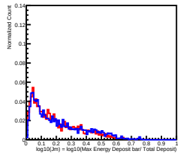
Deposit Energy[1584.89GeV, 2511.89GeV] in L2
