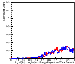
Deposit Energy[1584.89GeV, 2511.89GeV] in L7
