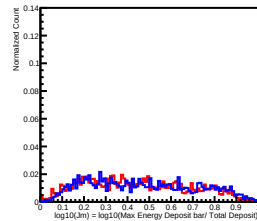
Deposit Energy[1584.89GeV, 2511.89GeV] in L3
