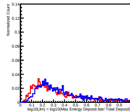
Deposit Energy[1584.89GeV, 2511.89GeV] in L13
