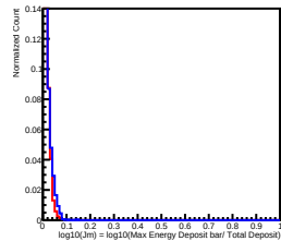
Deposit Energy[1584.89GeV, 2511.89GeV] in L0
