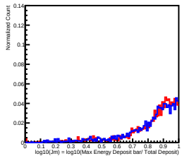
Deposit Energy[1584.89GeV, 2511.89GeV] in L6
