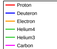
IncidentParticle 10GeV
