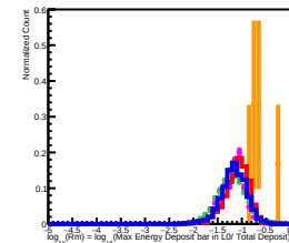
20 GeV incident in L3
