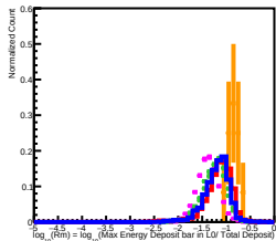
50 GeV incident in L4
