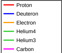
IncidentParticle 60GeV
