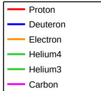
IncidentParticle 800GeV
